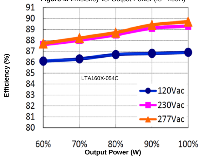
Figure 6: Efficiency vs. Output Power ( I_o=3.80A )
