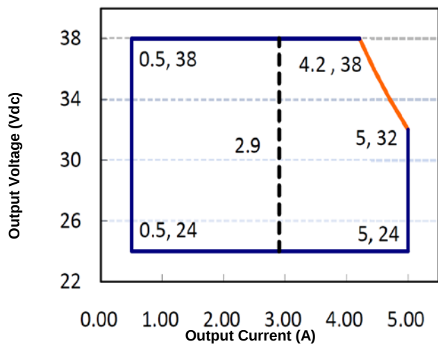
Figure 1: Typical V-I Characteristic Curve (LTA160X-038C)
