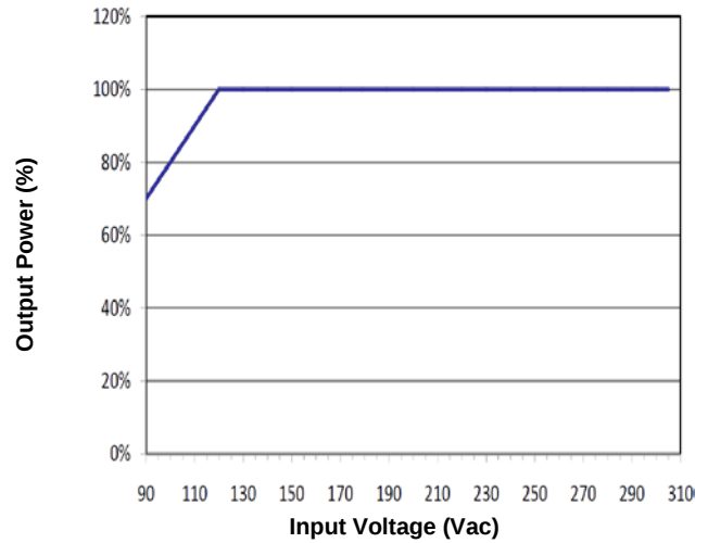
Figure 11: Output Power vs. Input Voltage
