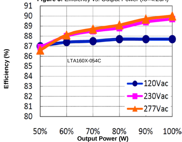
Figure 7: Efficiency vs. Output Power ( I_o=2.96A )
