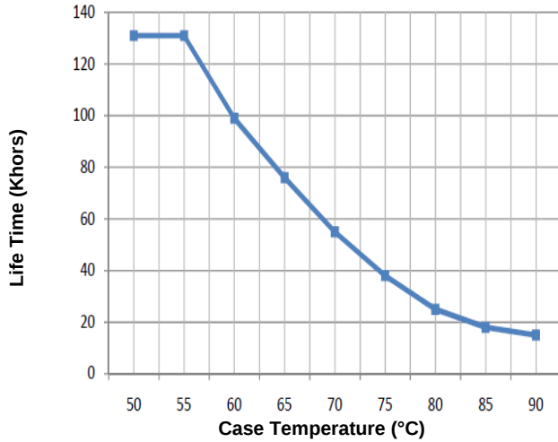
Figure 12: Life Time vs. Case Temperature
