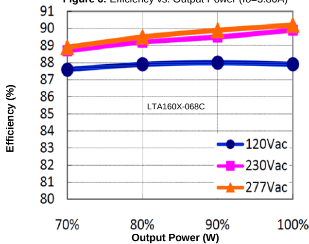
Figure 8: Efficiency vs. Output Power ( I_o=2.85A )
