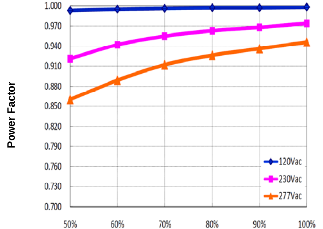
Figure 13: Power Factor vs. Output Power
