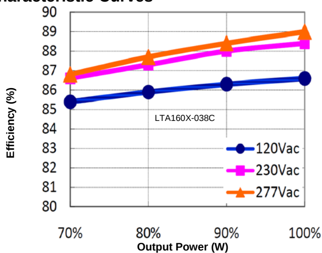
Figure 4: Efficiency vs. Output Power ( I_o=4.00A )
