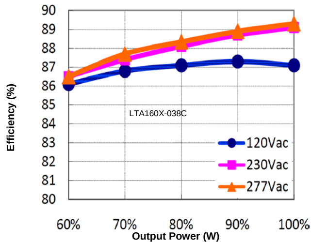
Figure 5: Efficiency vs. Output Power ( I_o=4.20A )
