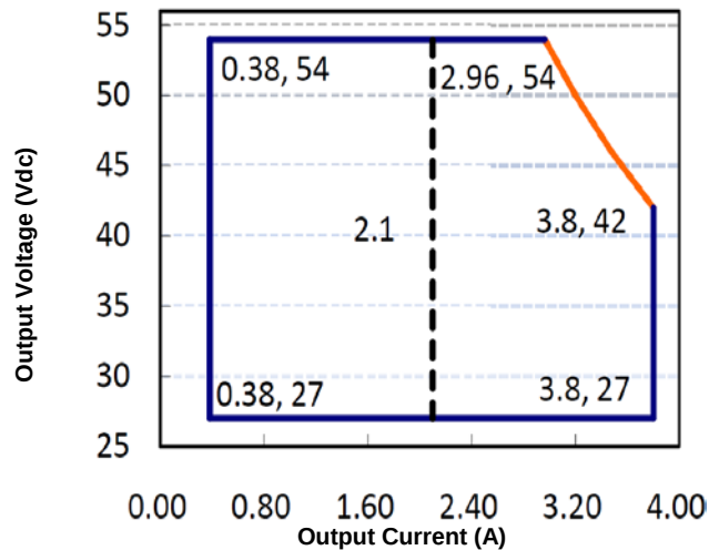
Figure 2: Typical V-I Characteristic Curve (LTA160X-054C)
