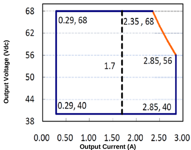
Figure 3: Typical V-I Characteristic Curve (LTA160X-068C)
